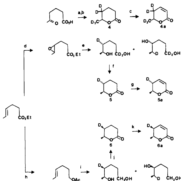
Scheme II d
